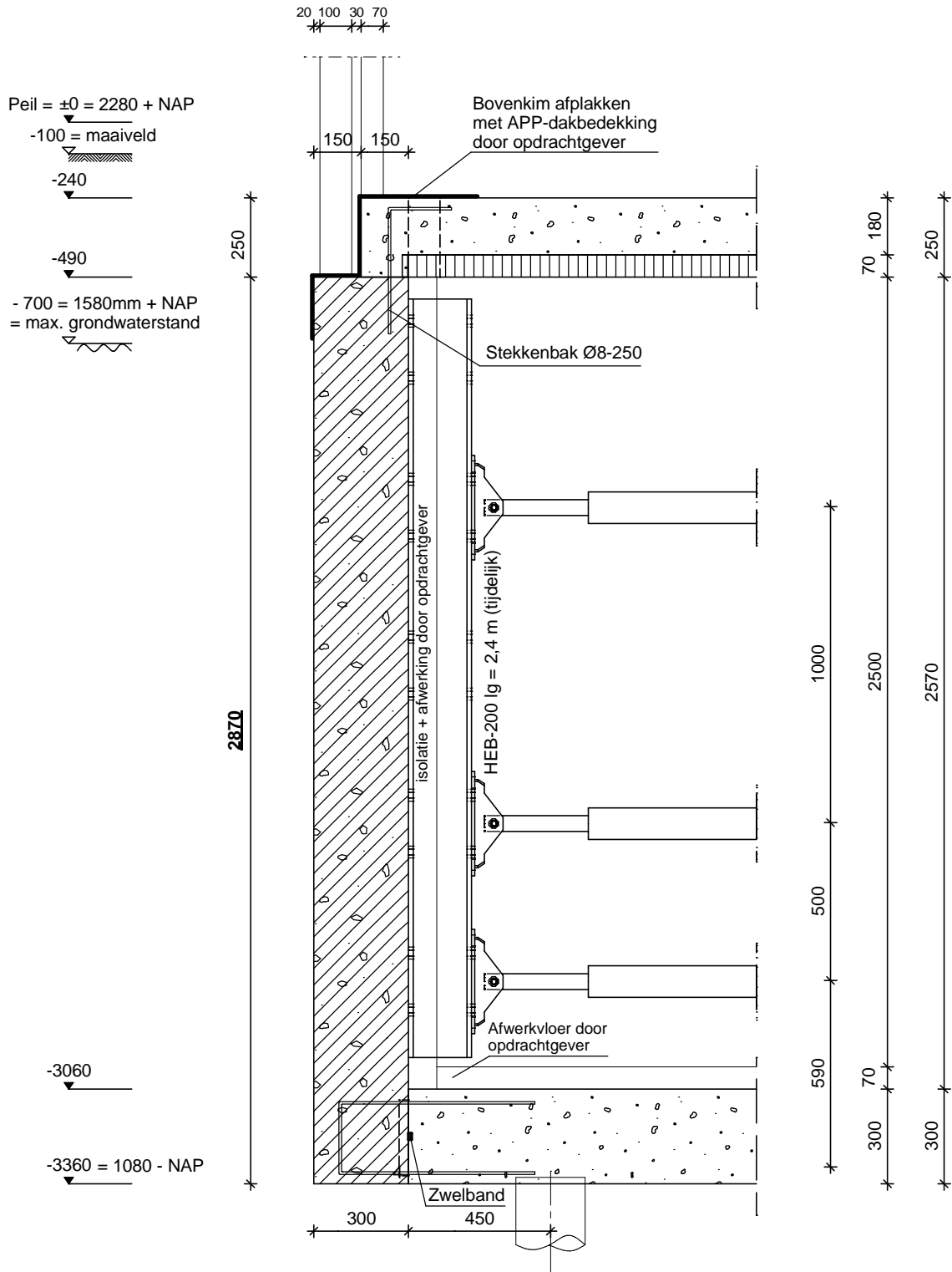
Principe detail wand afzinkkelder
